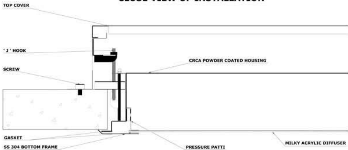
CLOSE VIEW OF INSTALLATION
