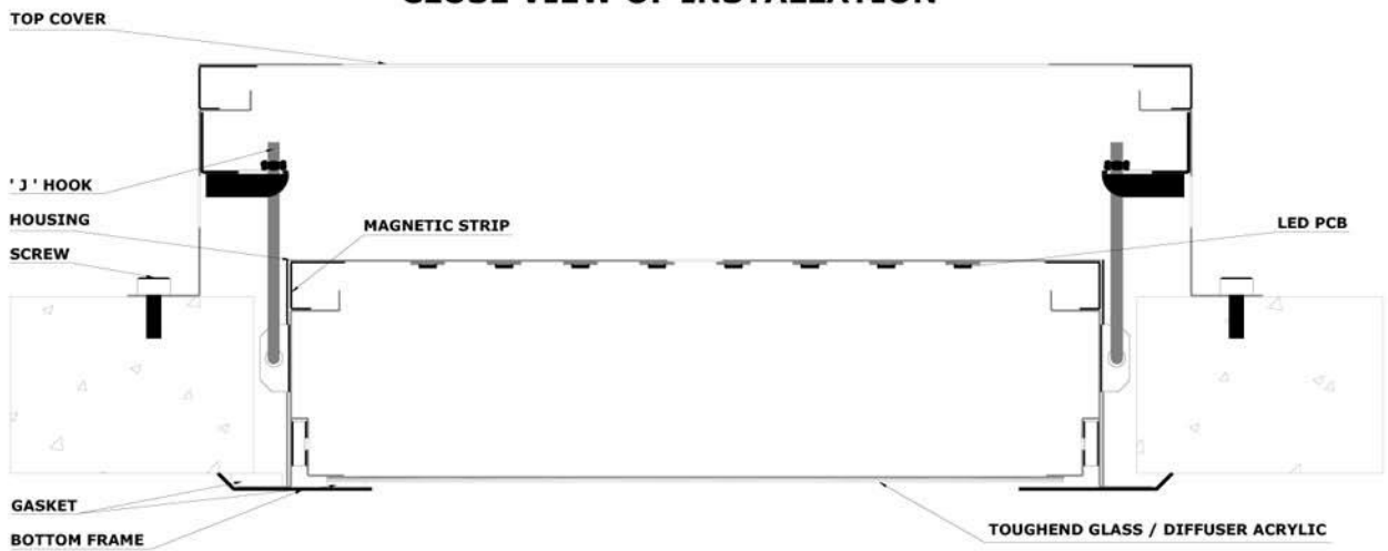
CLOSE VIEW OF INSTALLATION
