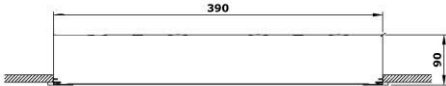
CLOSE VIEW OF INSTALLATION
