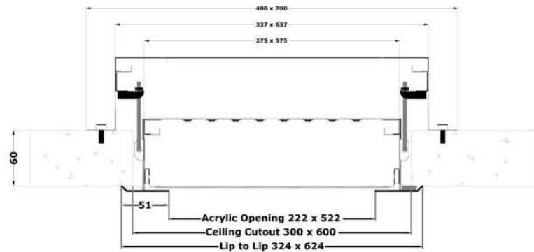
MOUNTED & DIMENSION VIEW
