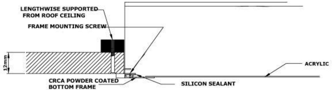
CLOSE VIEW OF INSTALLATION
