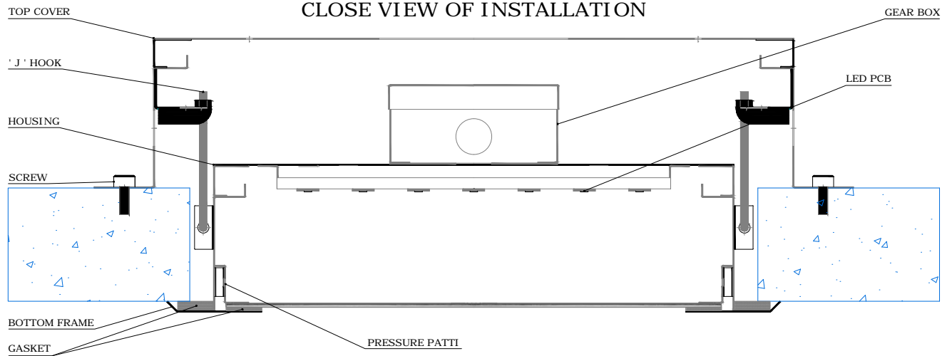
CLOSE VIEW OF INSTALLATION
